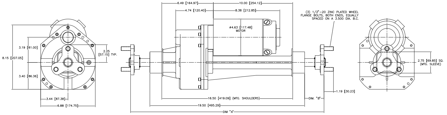
MODEL 318 TRANSAXLE
